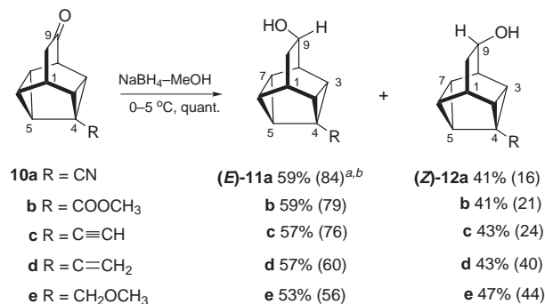
Scheme 2 a Values in parentheses indicate E : Z ratios for hydride additions to nornsnoutanones 9a–e . b Ratios based on 1 H NMR integrals of crude mixture (±5%).
